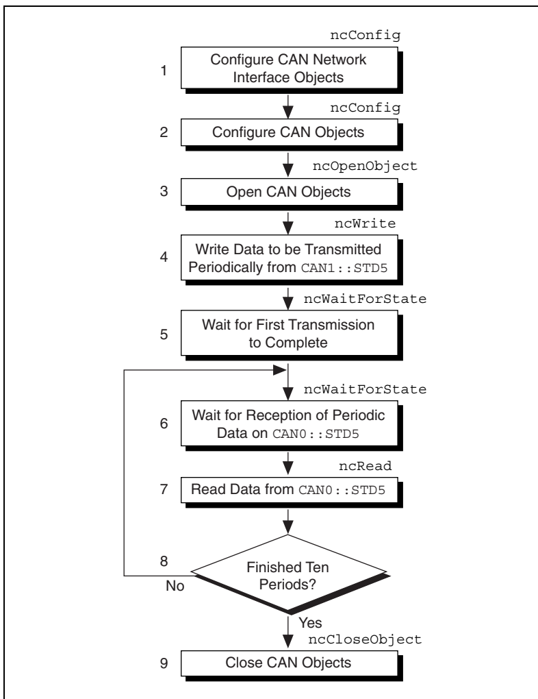
Figure 4-1. Program Flowchart for Example 1
